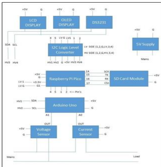
Fig10. Circuit Diagram
