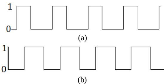
Fig. 3(a) and (b) Gating pulses to the switches S_1 and S_2
