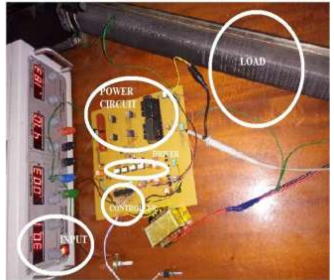
Fig. 17. Experimental Setup
