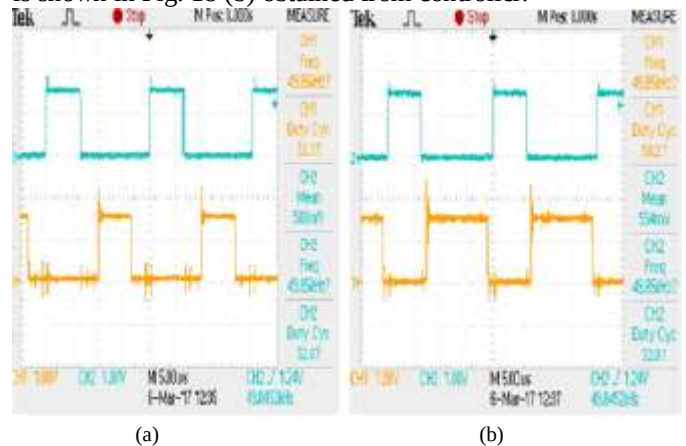
Fig. 18. (a) 180 Degree Pulse and (b) Complementary Pulse
