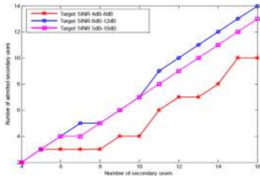
Figure 3: Total users Vs Number of admitted secondary users under variable bounded SINR constraint
