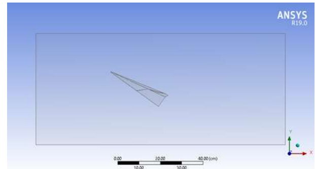
Fig.3 Fluid domain of typical dart.
