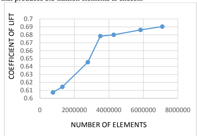
Fig.4.Mesh independence study.
