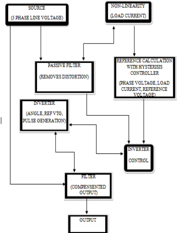
Fig 4a Flow diagram of the process
