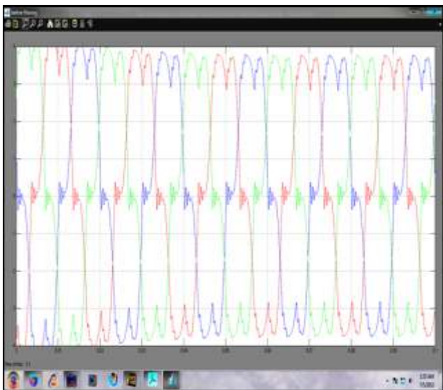
Fig. 6 Wave forms of Supply Current (A) without filter
