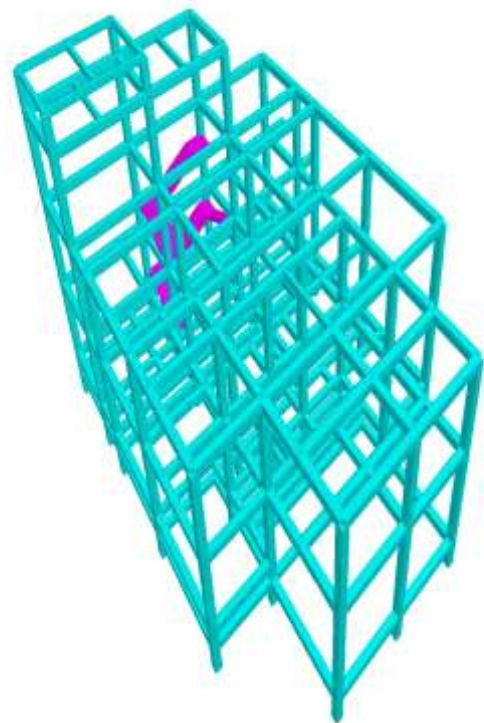
Fig 3 Staad 3D model
