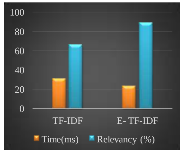
Figure 2: Performance analysis for text file
