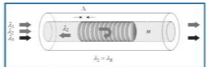
Fig 1 Working Principle of FBG
