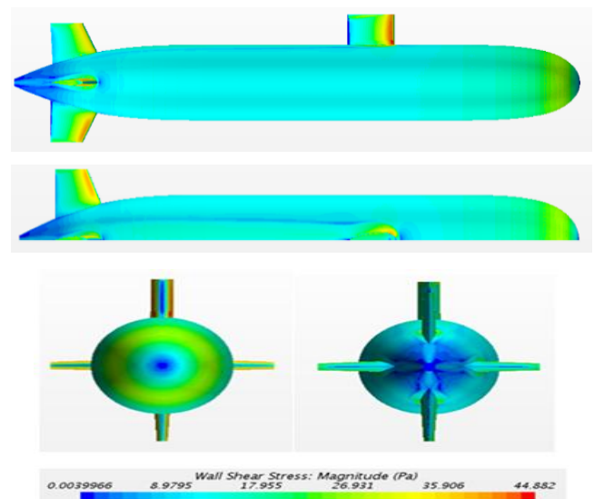
Fig.6. Shear stress distribution along the hull at speed V=3,05\text{m/s}
