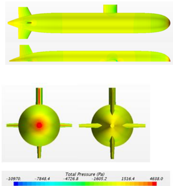
Fig.8. Pressure distribution along the hull at speed V=3.05\text{m/s}
