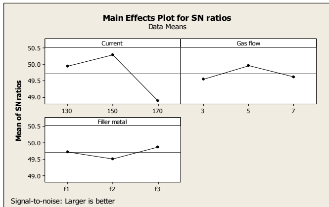
Fig. 8: SN ratios graph for Tensile Strength Testing
