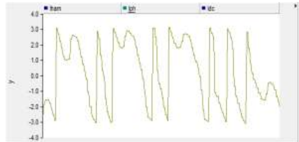
3rd phase current, when, n = 3 .
