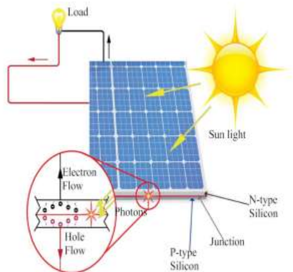
Figure 1 Conversion mechanism of solar radiation into electricity
