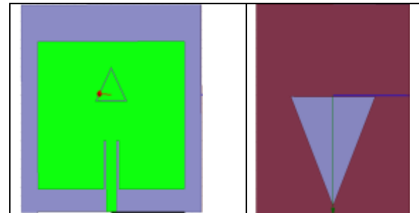
Fig. 2. Top and bottom view of miniaturised rectangular microstrip patch antenna with a resonance frequency of 2.4 GHz
