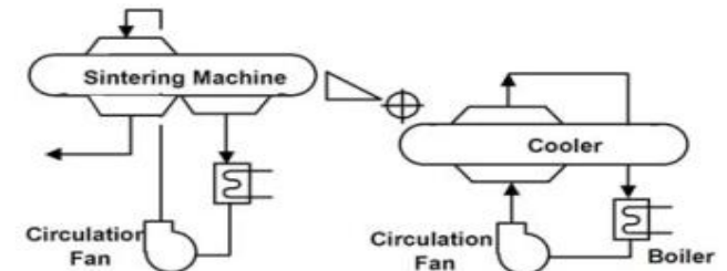
Case-3: Sinter & Cooler WHRS
