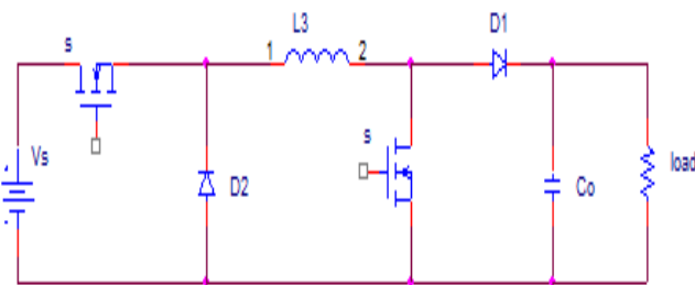
Fig.5 Circuit Diagram of NIBB Converter
