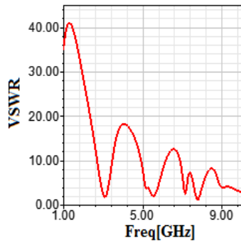
(b) 1st iteration stage
