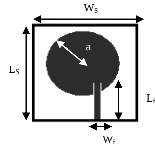
FIG. 1. (A) 0 th ITERATION STAGE OF CIRCULAR FRACTAL ANTENNA,
