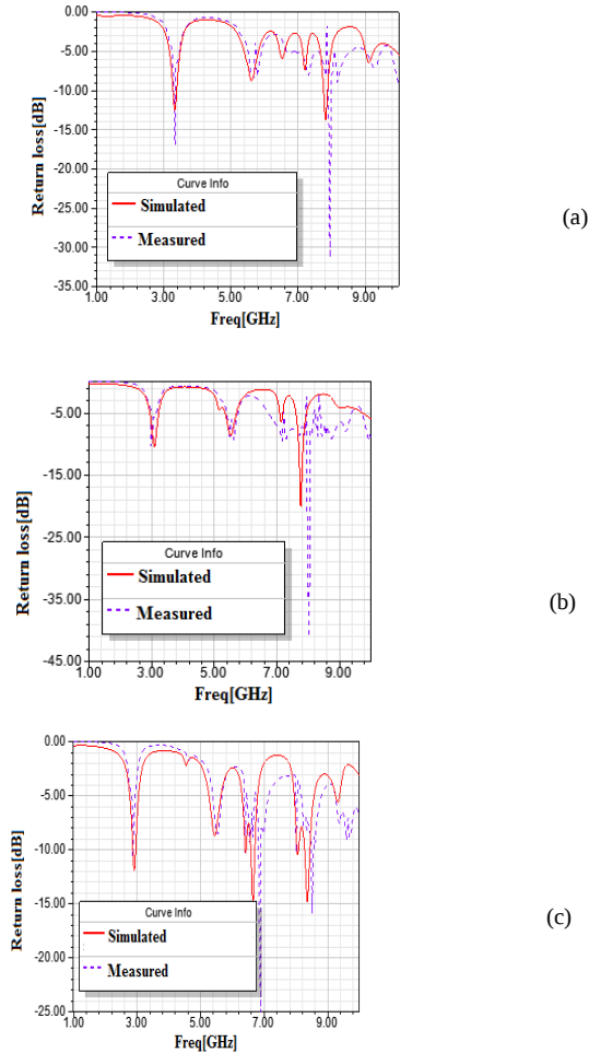
Fig. 9. Simulated and measured return loss vs. frequency plot of (a) 0 th iteration (b) 1 st iteration (c) 11 th iteration
