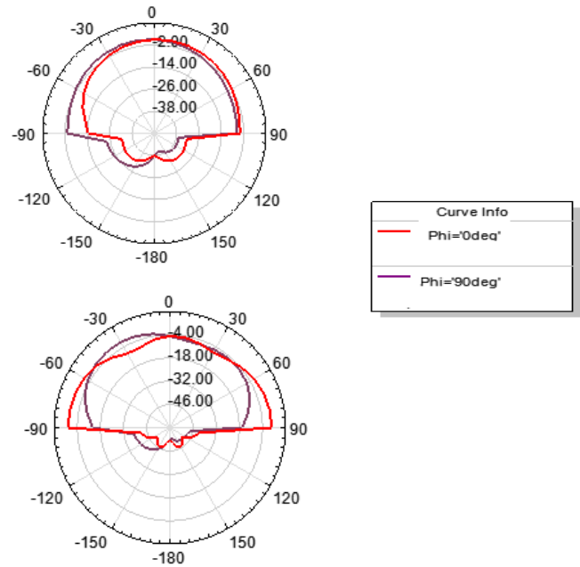
Figure 4. Simulated radiation pattern of 0 th iteration at (a) 3.34GHz (b) 7.81GHz
