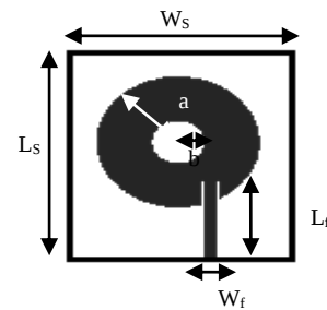
(B) 1 st ITERATION STAGE OF CIRCULAR FRACTAL ANTENNA
