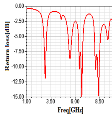
(c) IIInd iteration stage
