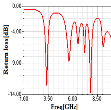
Fig. 2. Simulated return loss vs. frequency plot of (a) 0 th iteration stage,
