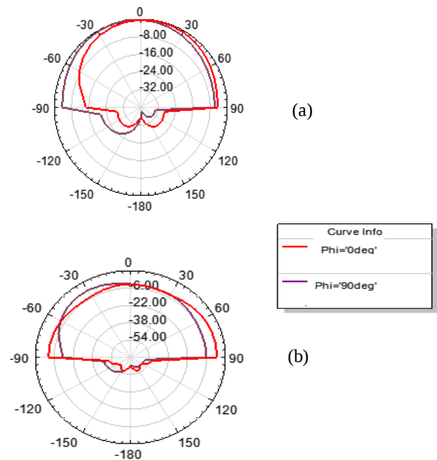
Figure 4. Simulated radiation pattern of 0 th iteration at (a) 3.34GHz (b) 7.81GHz
