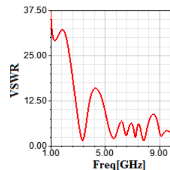
Figure 3. Simulated VSWR of (a) 0th iteration stage,
