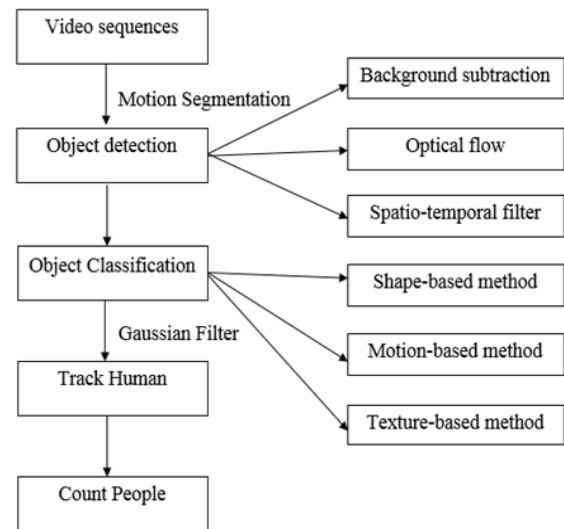
Fig. 1. People Counting Block Diagram
