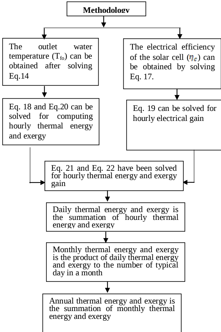
Fig.4 Methodology flow chart for the analysis of Cu/Al base PVT water collector
