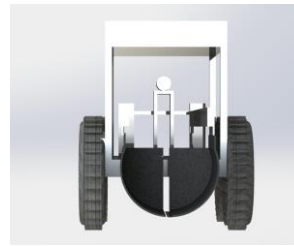
Fig.2 Front View
