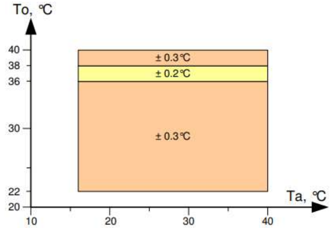
Fig 3: Medical Accuracy of MLX90614
