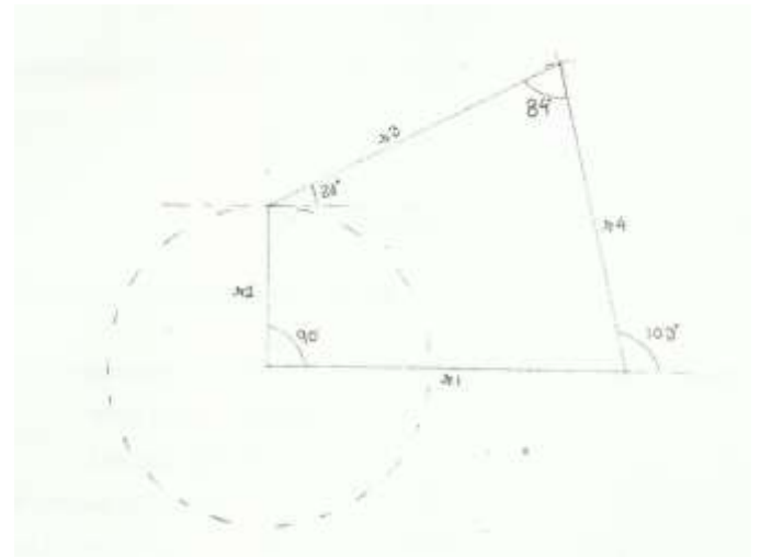
Fig. 4. Position Analysis ( \theta_1 = 90^\circ degree)
