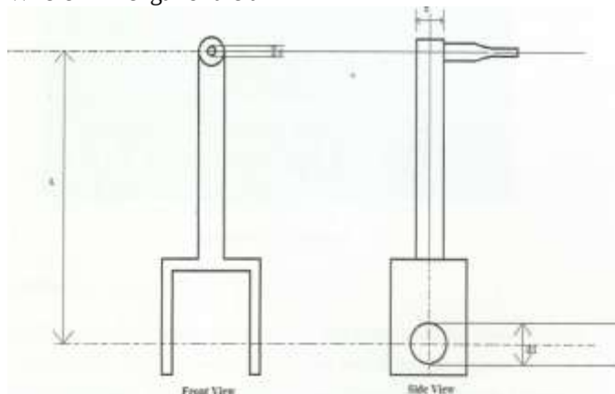
Fig.8. Oscillating Arm
