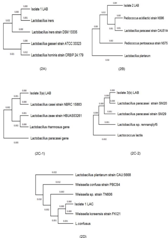
Figure 2 Phylogenetic tree constructed using MEGA X software for LAB isolates
