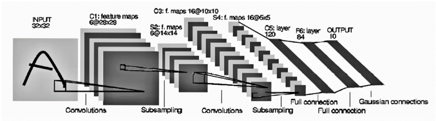
Fig. 1. Typical CNN(LeNet) [3]
