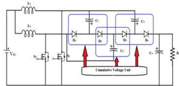
Fig. 2. Circuit Diagram of High gain Interleaved Boost Converter
