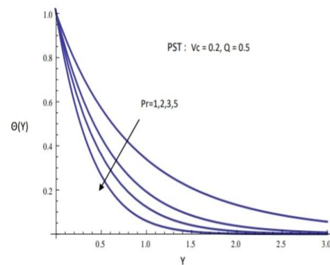
Fig. 8: Effect of Pr on temperature profile \Theta(Y) in PST case.
