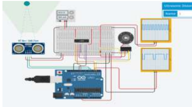
Fig. 2. Tinkercad PID Controller
