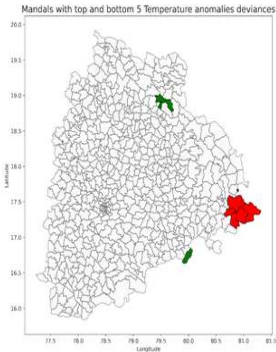
Fig 4. Telangana Mandal deviances in Temperature anomalies, positive values are highlighted in green and the ones with the least positive/ negative deviations were highlighted in red.
