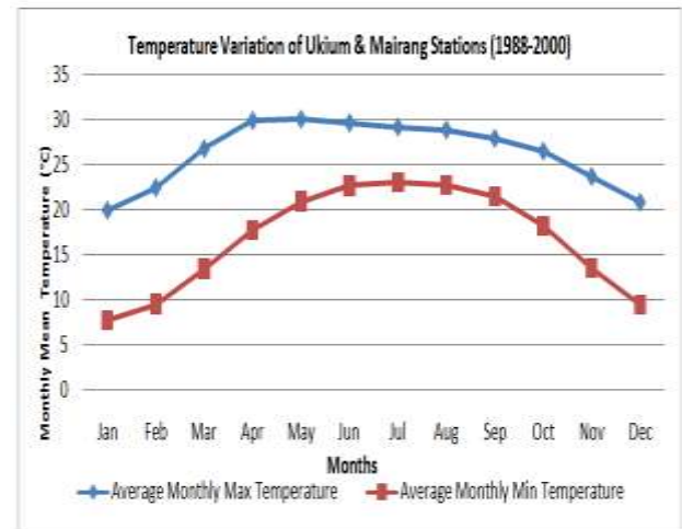
Fig 3: Monthly mean temperature (1988-2000)
