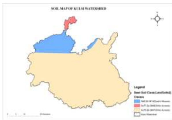
Fig 5: Kushi watershed soil classes
