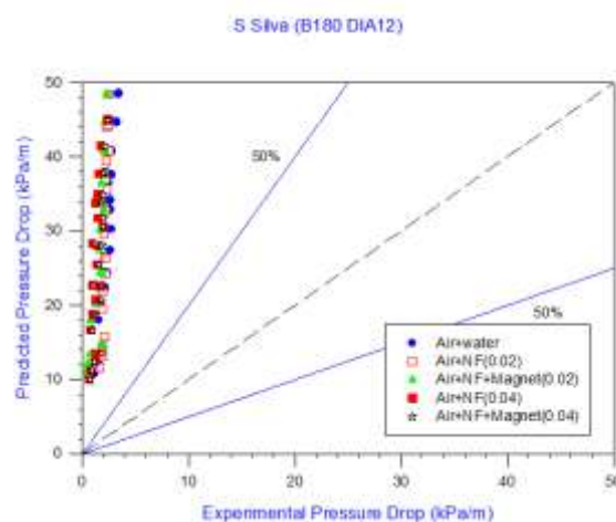
Fig. 7 Comparison of S Silva correlations with experimental data.
