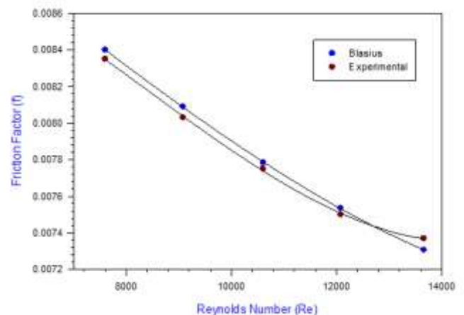
Fig 2. Comparison of experimental single-phase friction factor with Blasius correlation.
