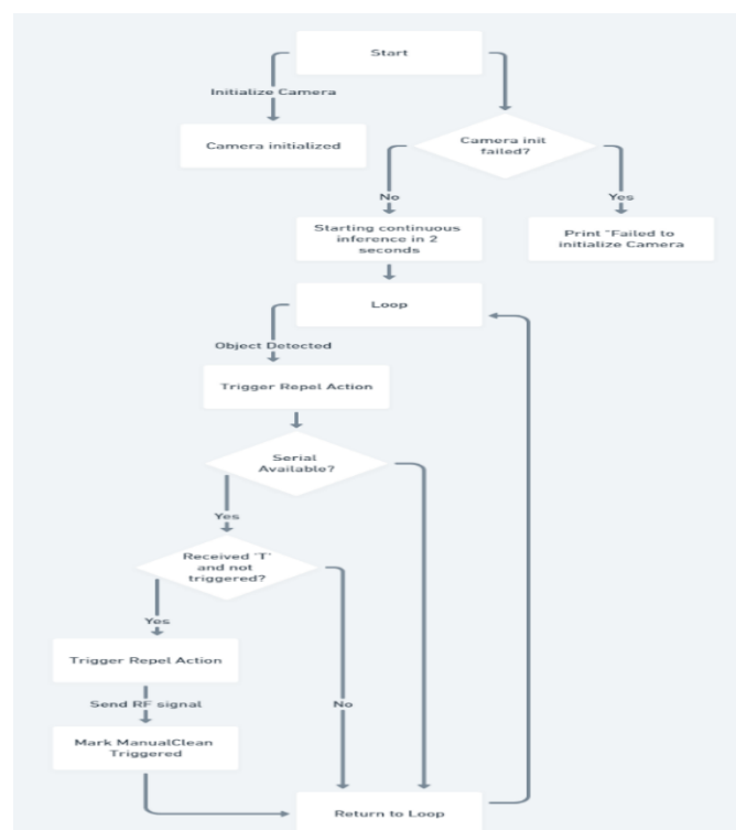
Fig. 1. ESP32 flowchart
