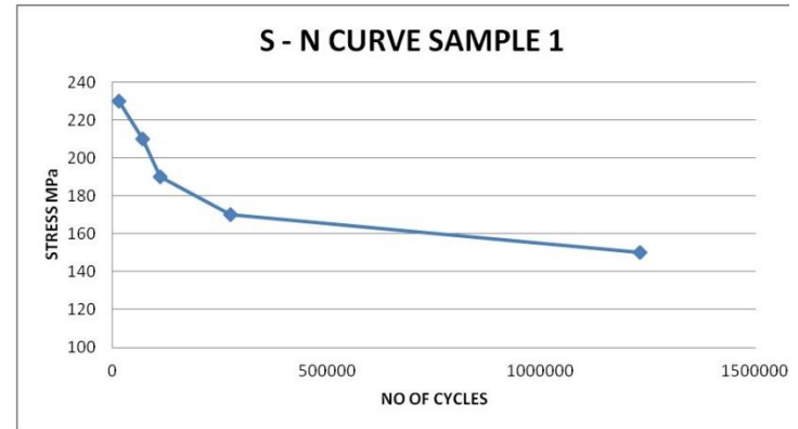
Fig 13 S-N Curve for Specimens before finishing
