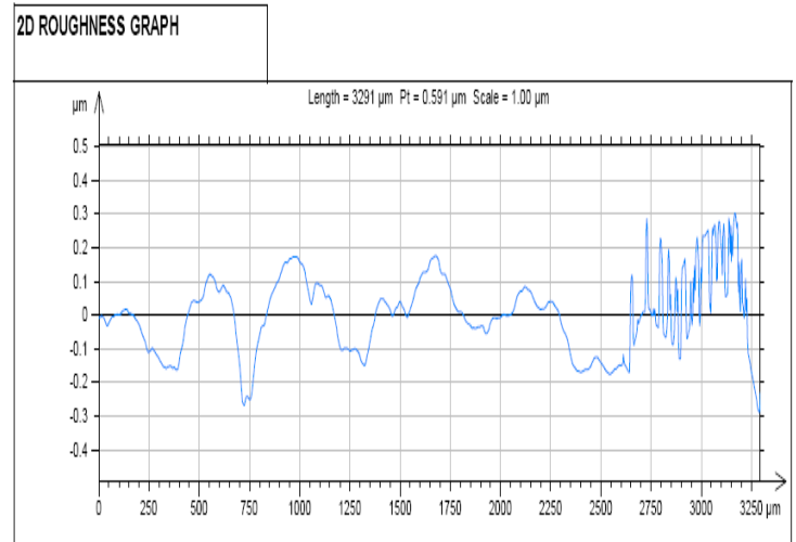
Fig 4 2D Roughness Graph
