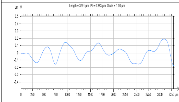
Fig 5 Filtering and waviness Graph
