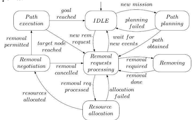
Figure 6: Overall machine logic flowchart (Draganjac et al., 2016)
