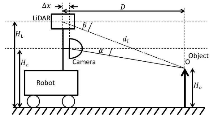
Figure 2: Schematic diagram of AGV (De Silva et al., 2018)
