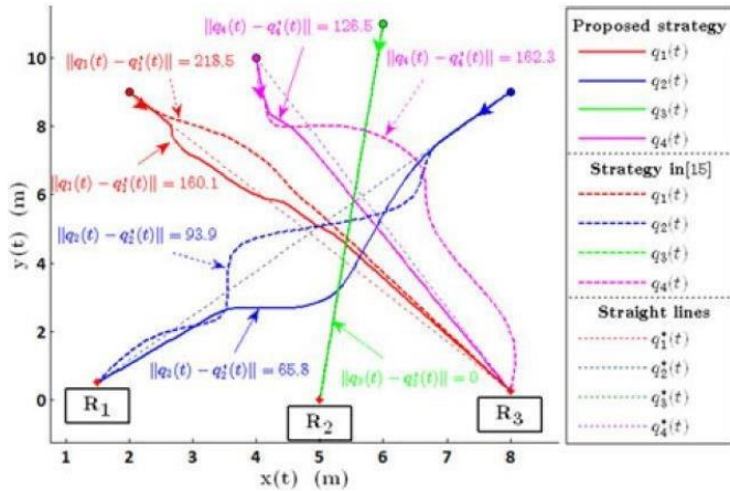
Figure 18: Graph of path planning simulation (Demasure et al., 2017)
