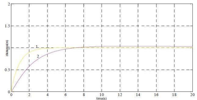
Figure 8: Step Response Graph (Zhou et al., 2018)
