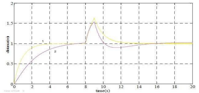
Figure 9: Step disturbance Response Graph (Zhou et al., 2018)
