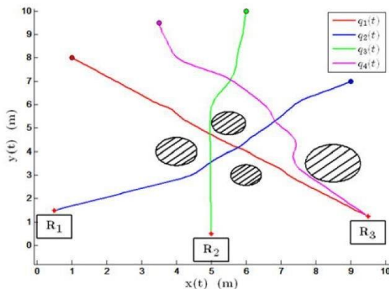
Figure 19: Path planning with obstacles (Demasure et al., 2017)
