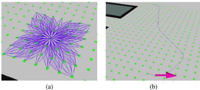
Figure 5: (a) Possible paths from given center point (b) Example of computed path based on lattice points (Draganjac et al., 2016)
