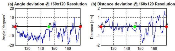
Figure 10: Angular and linear error (Oliveira et al., 2019)
