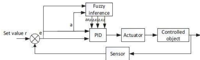
Figure 1: Fuzzy logic PID control system (Zhou et al., 2018)
