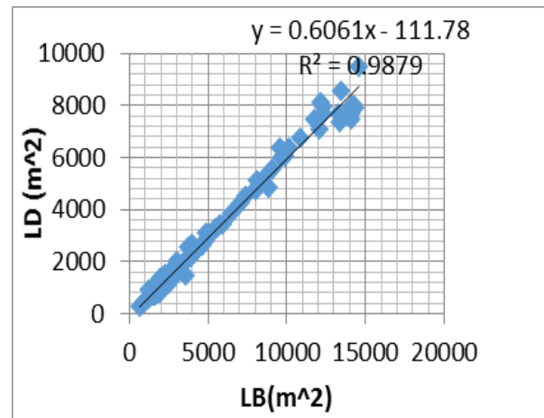
FIG. 16: VESSEL LxD TO LxB
