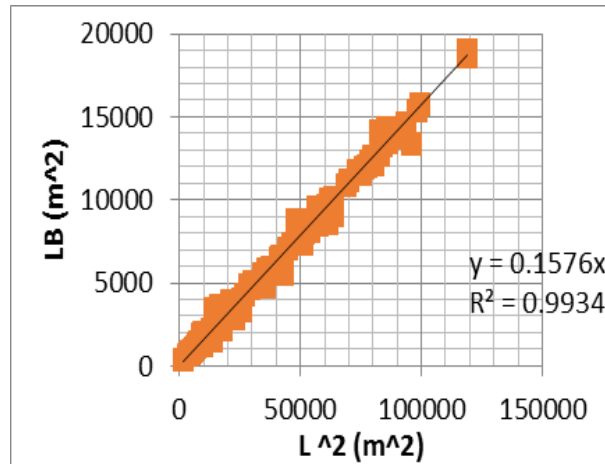
FIG. 11: LxB TO L2 REGRESSION.
