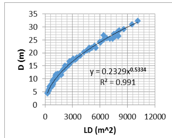
FIG. 18 VESSEL DEPTH TO LxD REGRESSION
