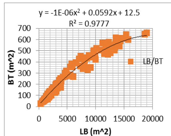
FIG. 24 VESSEL BEAMxDRAFT BxT TO Lx REGRESSION.
