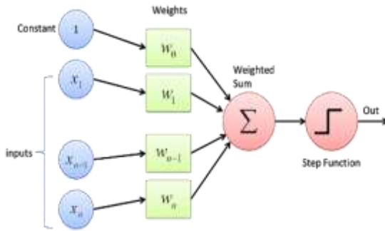
Fig. 2. Perceptron Structure [13]
