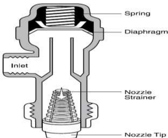
Figure 11 Nozzle design
