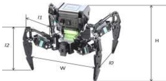
Fig. 8 Proposed "Lean-Agriot" with twelve degrees of freedom
