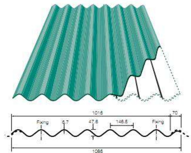
Fig 1. – Reinforcement Sheet
