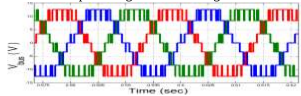
Fig. 21. Three Phase Output Voltage
