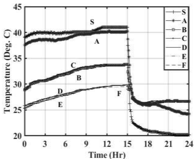
Fig. 5. Temperature variation inside a brick model
