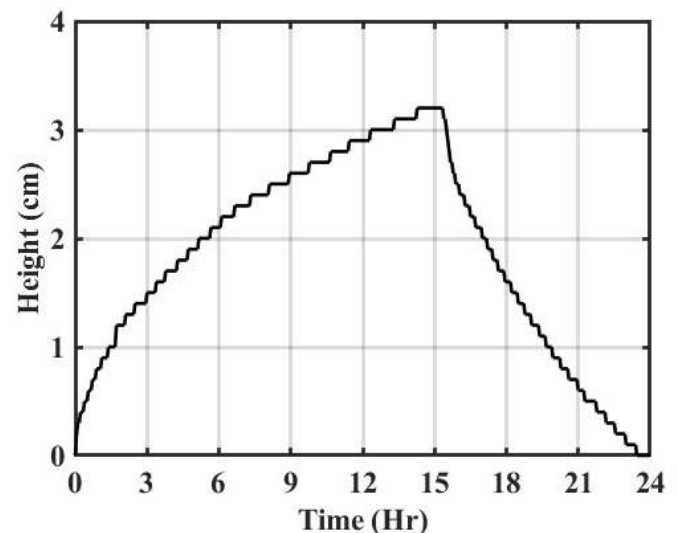
Fig. 6. PCM height variation with respect to the time
