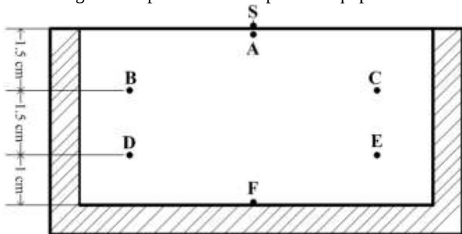
Fig. 2. Position of thermocouples inside a brick model
