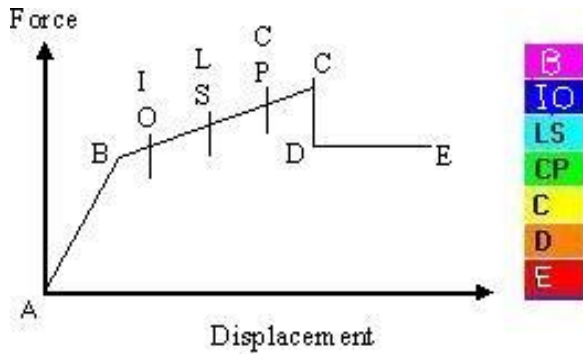
Fig.1. Load-displacement curve
