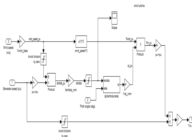
Fig..5 Simulink model of wind turbine
