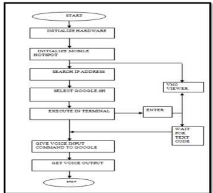
Figure 3: Flowchart for Google assistant
