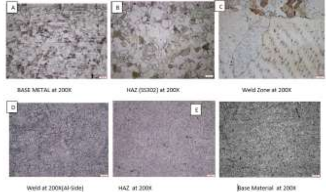
Fig. 11. Sample-2 micro structure with different specimens in 70 Amps
