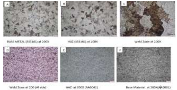
Fig. 14. Sample-3 micro structure with different specimens in 70 Amps
