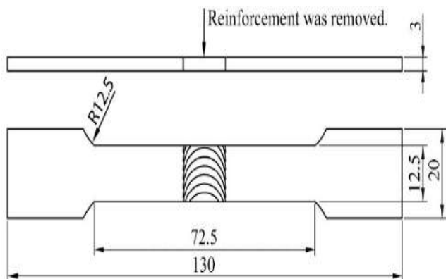
Fig. 1. Shows the preparation drawing for tensile test
