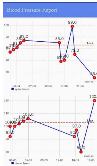
Fig. 6.6 Reports Screen
