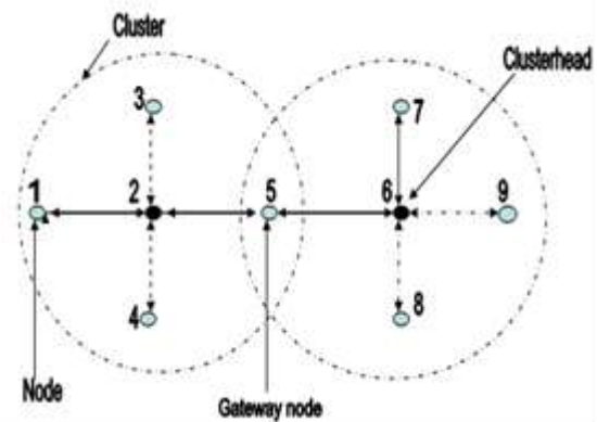
Fig. 1 Clustering
