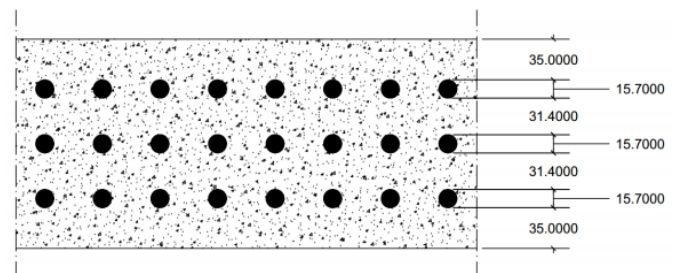
Figure 2 c/s of bottom flanges
