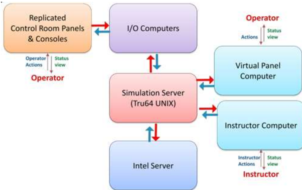
Fig. 1. Hardware Architecture
