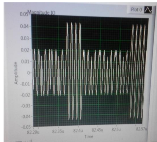
Fig 10: output waveform of QAM in front panel
