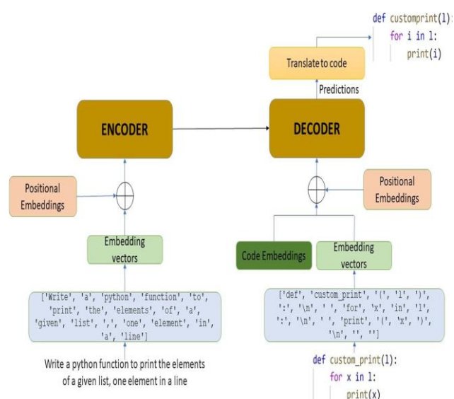
Figure 3:Architecture of the final model.
