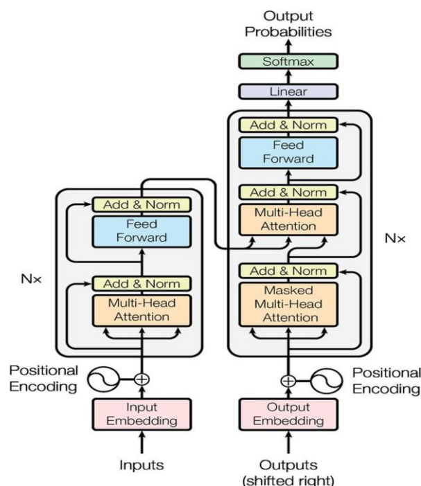
Figure 2: The Transformer Model
