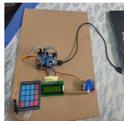
Fig.3.1 System Setup
